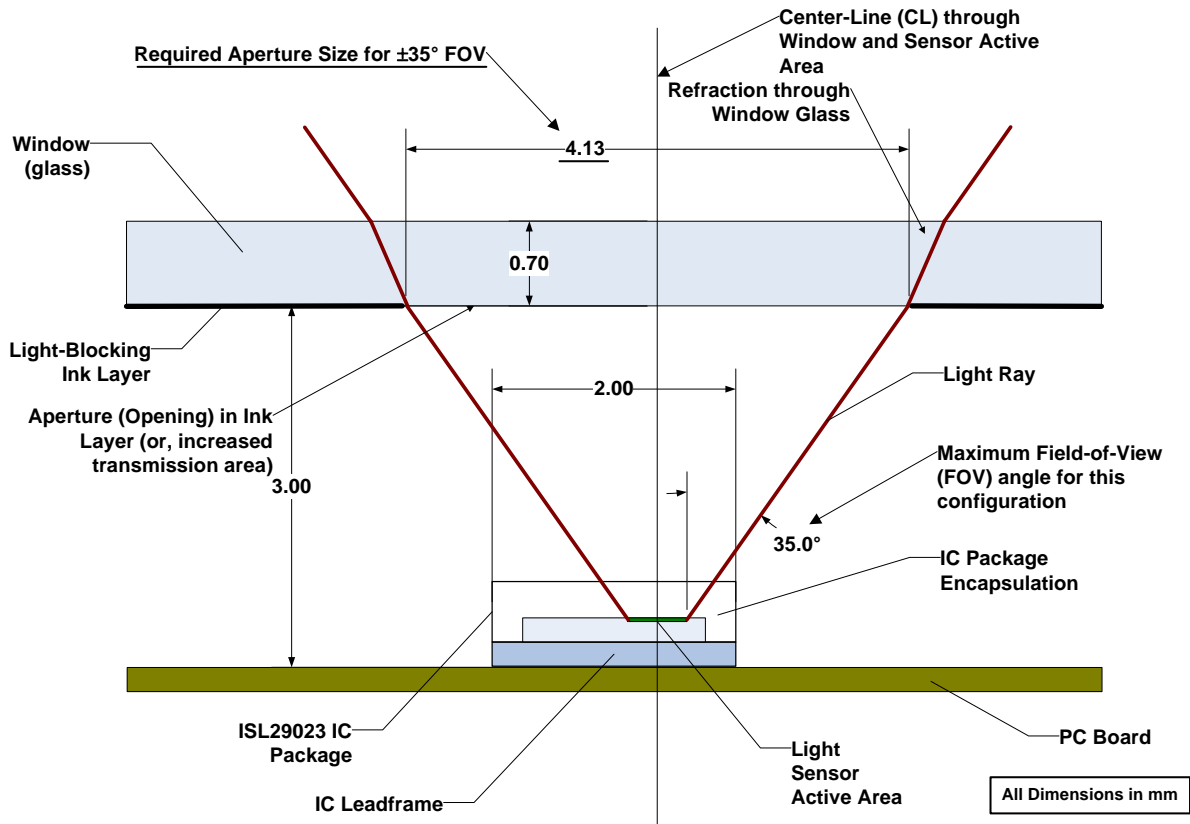
FIGURE 10. SOFT APERTURE DETAILED DRAWING
