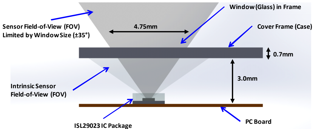
FIGURE 4. REFERENCE MODEL SIDE VIEW
